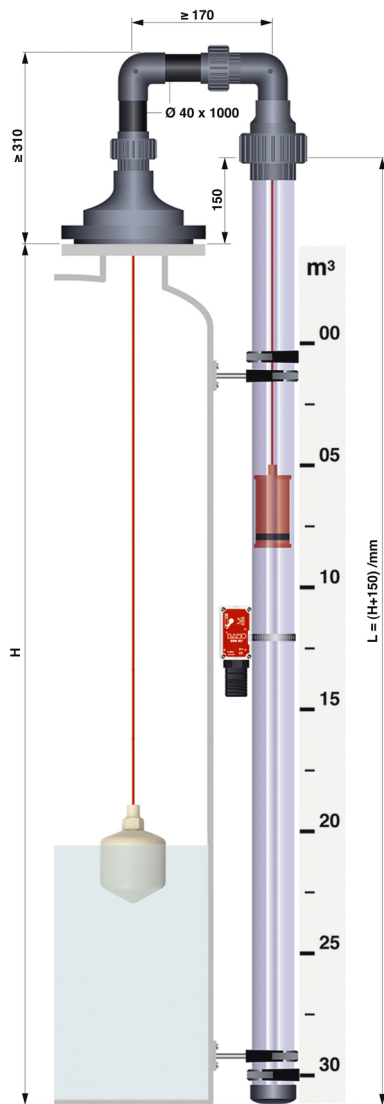
Plastic version with graduated ruler option
