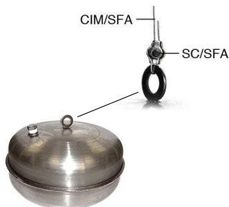
Float and cable in stainless steel (variant)
