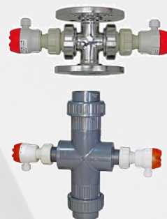
TURBISWITCH GA 50...30000 FAU for use with GS5
