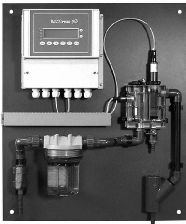
Example of a complete assembly
