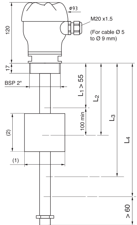
Model BSP 2"
