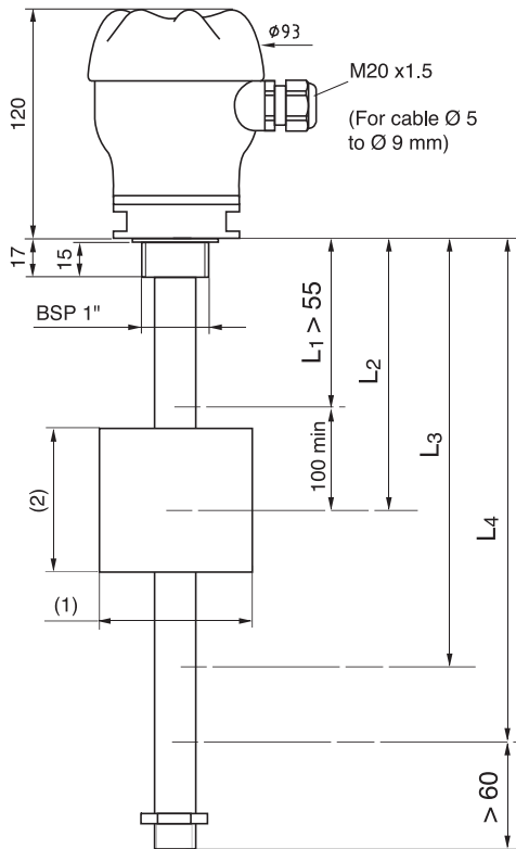
Model BSP 1"
