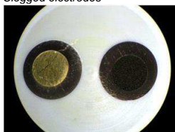
Dark: counter electrode Bright: measuring electrode
