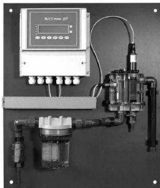
Example of a complete assembly
