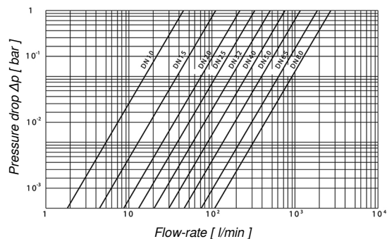
SV 95: Pressure drop vs. flow-rate
