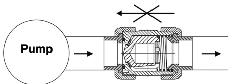
Check valve function ( SV95 )
